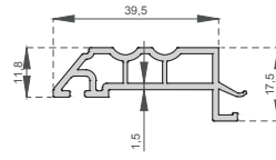
Motifli Pervaz Profili Patterned Architrave Profile A-1011
