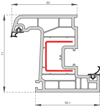
Kanat Profili Sash Profile C-7104
