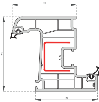
Kanat Profili Sash Profile C-7004
