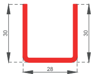
Kanat Profili Destek Sacı Sash Profile Reinforcement Steel
