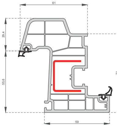
Damlıklı Kanat Profili Window Sash With Drip Profile C-7005
