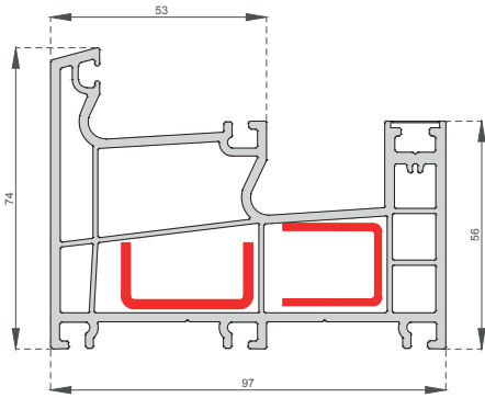
Dış Fix Kasa Profili Outside Fix Frame Profile CS-1004
