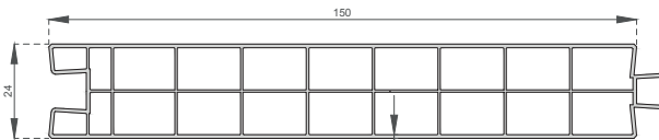
150'lik 24 mm Lambiri 150' 24 mm Panel A-1020
