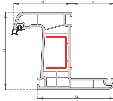
Pervazlı Kasa Profili Frame Profile With Architrave C-7002
