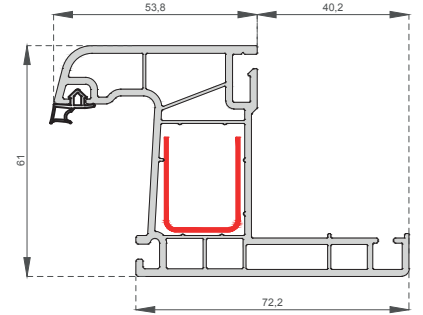
Pervazlı Kasa Profili Frame Profile With Architrave C-6006
