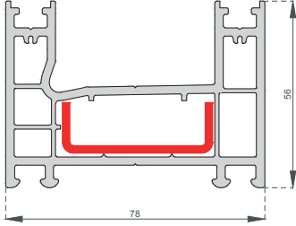
Kasa Profili Frame Profile CS-1001
