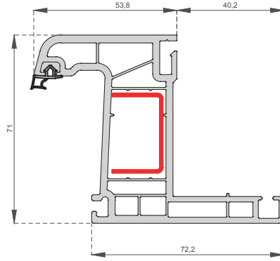
Pervazlı Kasa Profili Frame Profile With Architrave C-7102
