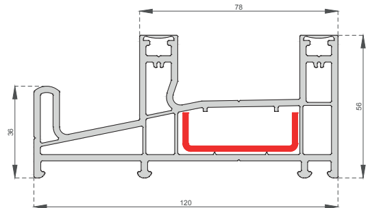
Sineklikli Kasa Profili Frame Profile With Flyscreen CS-1007
