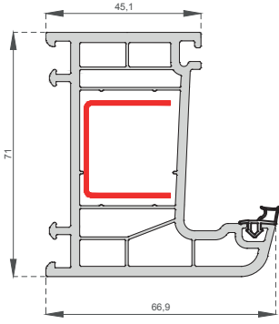
Kasa Profili Frame Profile C-7101
