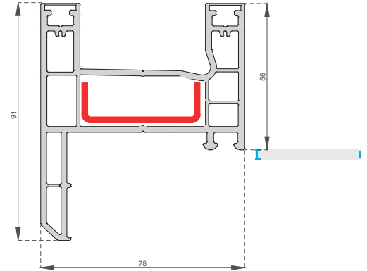
Pervazlı Kasa Profili Frame Profile With Architrave CS-1005
