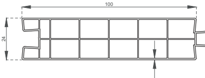
100'lük 24 mm Lambiri 100' 24 mm Panel A-1019
