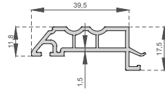
Motifli Pervaz Profili Patterned Architrave Profile A-1011
