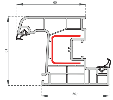
Kanat Profili Sash Profile C-6003
