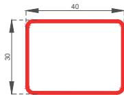
Kapı Destek Sacı Reinforcement Steel For Door
