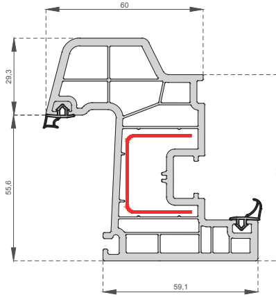
Damlıklıklı Kanat Profili Window Sash With Drip Profile C-7105
