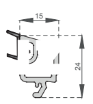
20 mm Cam Göre Çita Glazing Bead for 20 mm Glass CS-1012
