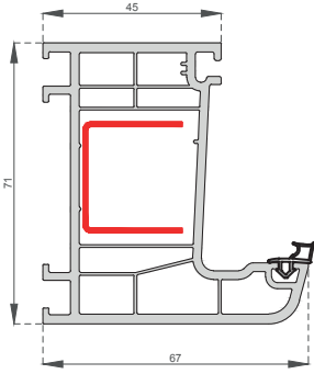
Kasa Profili Frame Profile C-7001
