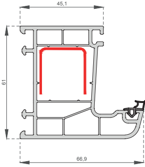
Kasa Profili Frame Profile C-6001
